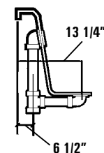
Rough-In Plumbing Measurements
